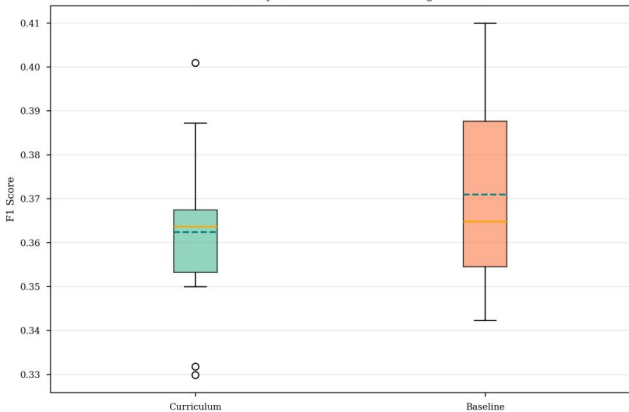
Seed Stability of Macro-F1 Across Training Methods
